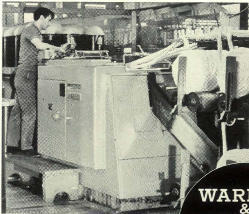
Wool fibers being prepared on Warner & Swasey SERVO-DRAFTER Automatic Leveling Draw Frame prior to twisting into yarn.
