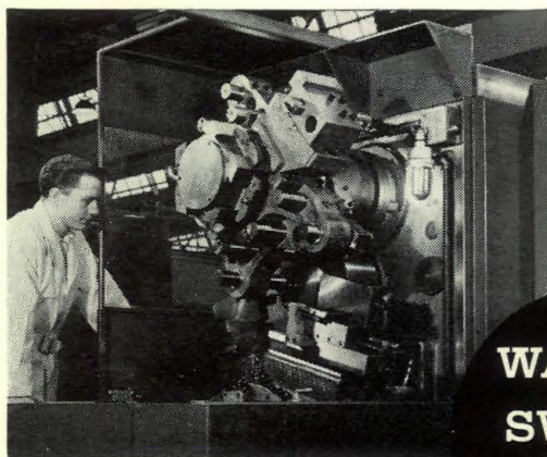
Cast iron flange for diesel electric locomotive on a 2-AC Automatic
