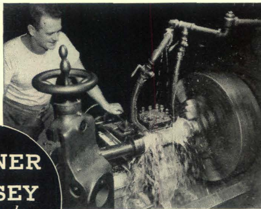
3-A Turret Lathe producing locomotive part
