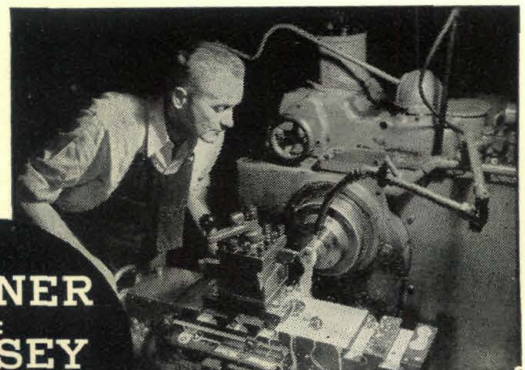
Turret Lathe producing parts for other turret lathes
