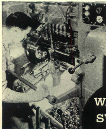
Multiple Spindle Automatic producing brass shell cases.
